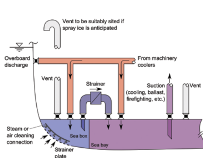
Figure 14: IMO suggested sea chest arrangement for slush and ice conditions
