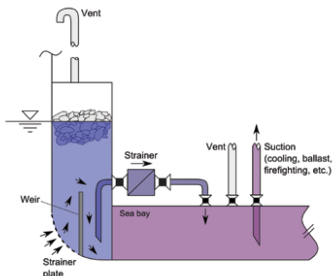
Figure 15: Typical sea chest arrangement for slush and ice conditions
